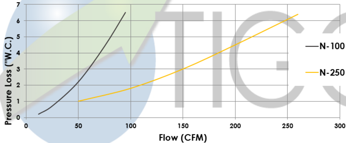
NIXTOX Drum Pressure Loss vs Flow Rate TIGG 4 x 10 Mesh Media (Dense Packed)
